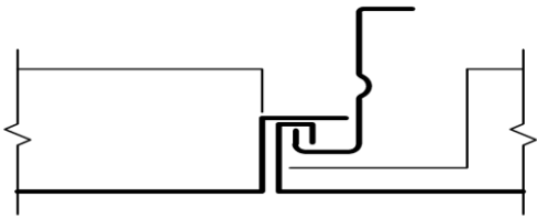
Fig. 2 – Example for a hook-on system
